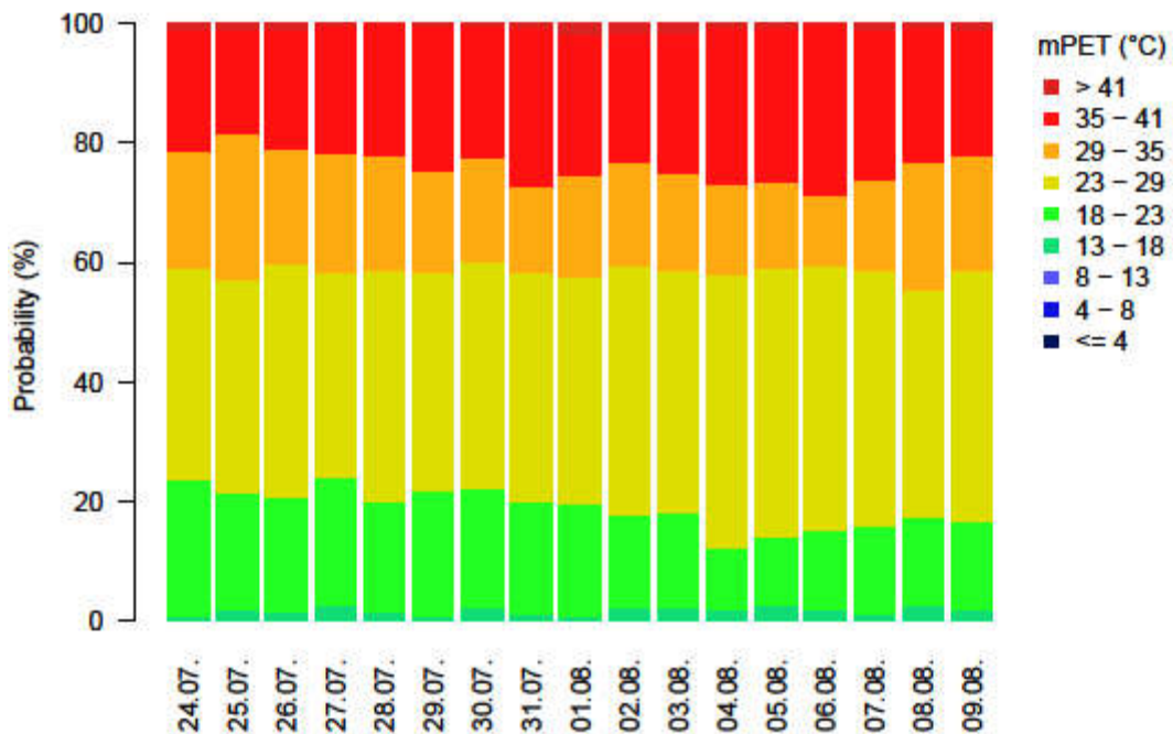
Figure 6. Frequency diagram showing the average occurrence of mPET classes for Tokyo for individual days in the range of the 24th of July and the 9th of August based on data of the years 1966 to 2018. The classes meet the thermal sensation classes stated in Table 2.
