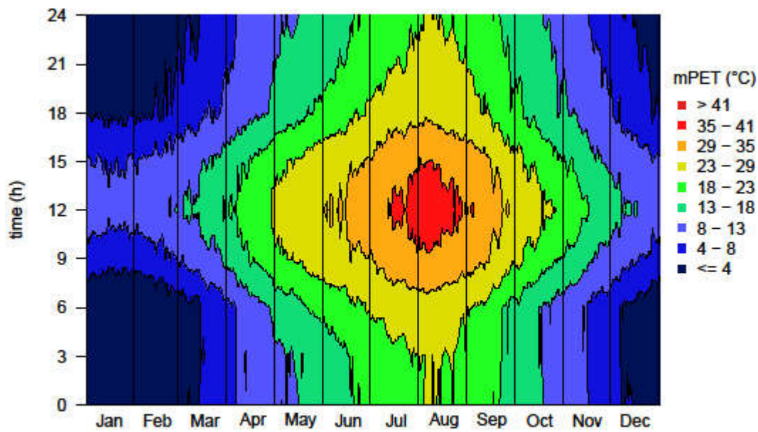
Figure 8. Temporal diagram for mPET for Tokyo during the period August 1966 to June 2018 (3 h resolution). The reference height for the results is 1.1 m. The sensation classes are defined in Table 2. The variation throughout the day can be seen in y-direction, while the variation over the year is given in x-direction.
