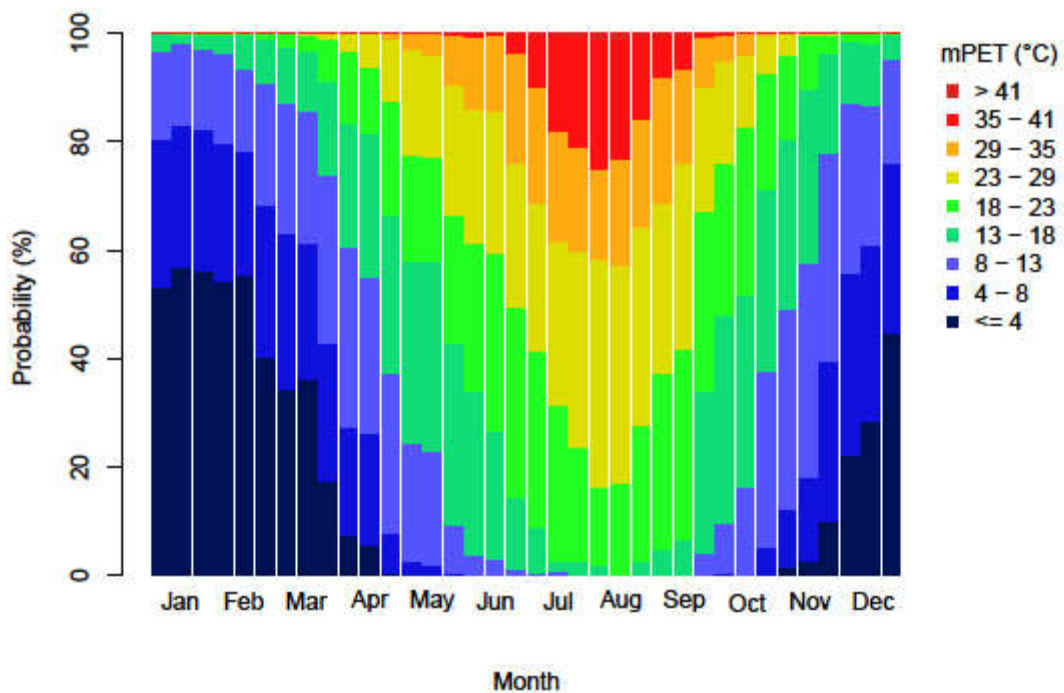
Figure 4. Frequency diagram (decades) showing the average occurrence of modified Physiological Equivalent Temperature (mPET) classes for Tokyo during the period August 1966 to June 2018 (3 h resolution). The reference height for the results is 1.1 m. The sensation classes are defined in Table 2.
