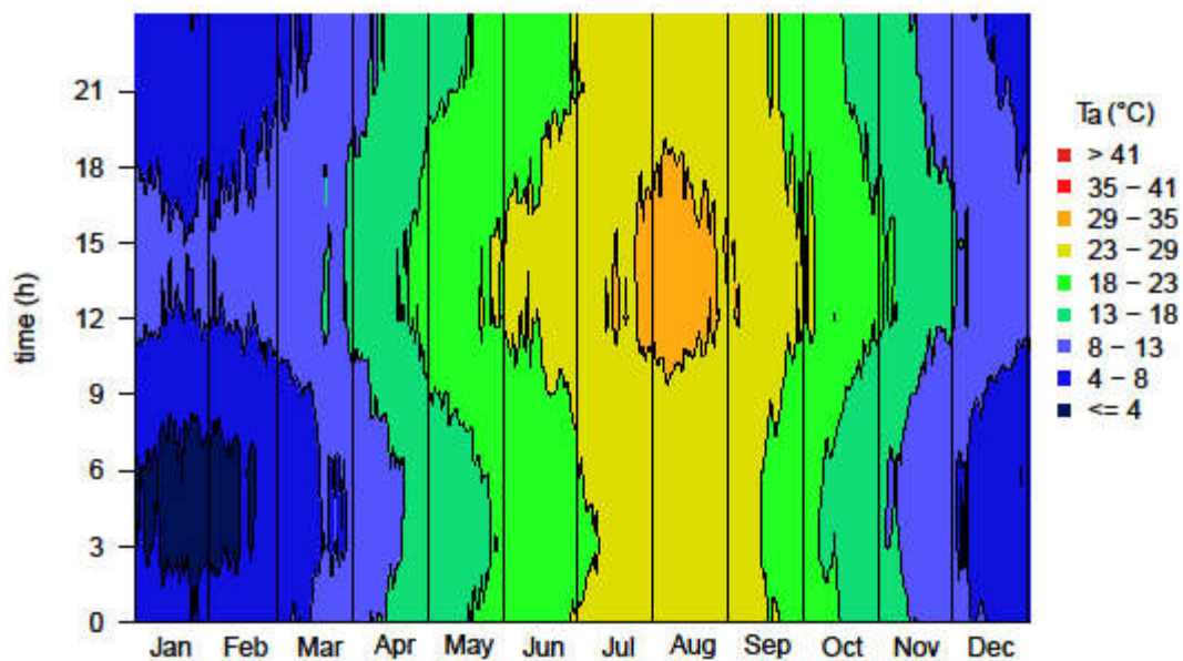
Figure 9. Temporal diagram for Ta for Tokyo during the period August 1966 to June 2018 (3 h resolution). The reference height for the results is 1.1 m. The sensation classes are defined in Table 2. The variation throughout the day can be seen in y-direction, while the variation over the year is given in x-direction.
