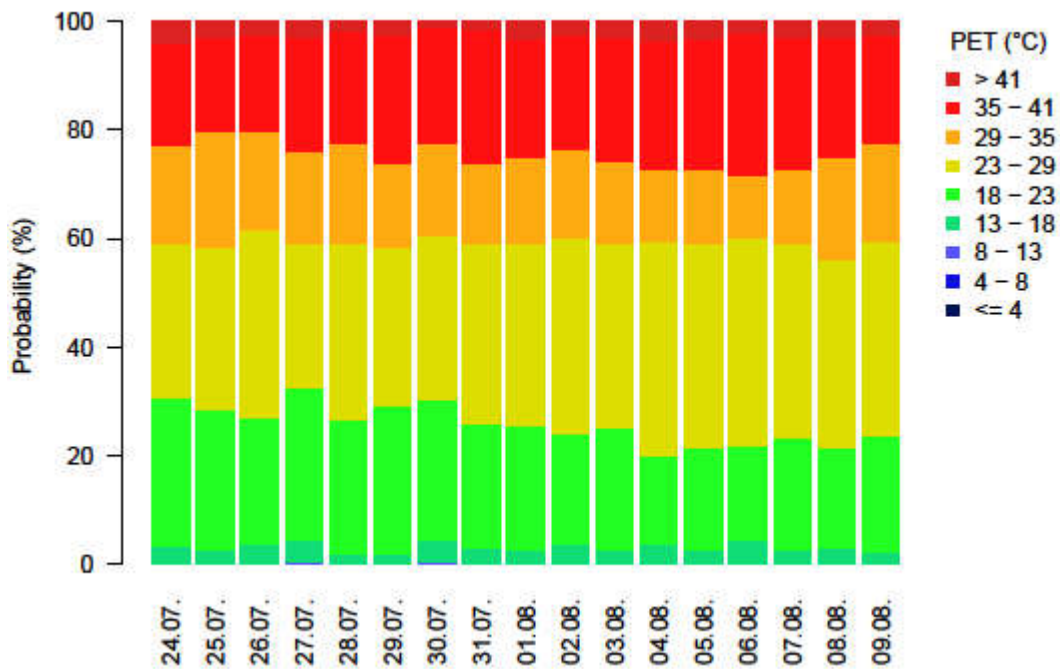
Figure 5. Frequency diagram showing the average occurrence of PET classes for Tokyo for individual days in the range of the 24th of July and the 9th of August based on data of the years 1966 to 2018. The classes meet the thermal sensation classes stated in Table 2.
