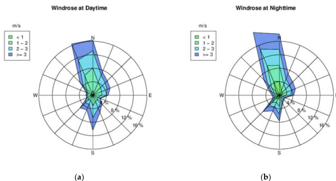
Figure 2. Wind roses showing the distribution of wind speed and direction in 1.1 m above ground for Tokyo City based on the period August 1966 to June 2018 at day (a) and nighttime (b).
