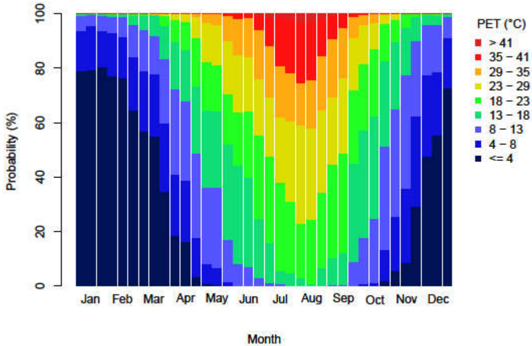
Figure 3. Frequency diagram (decades) showing the average occurrence of Physiologically Equivalent Temperature (PET) classes for Tokyo during the period August 1966 to June 2018 (3 h resolution). The reference height for the results is 1.1 m. The sensation classes are defined in Table 2.
